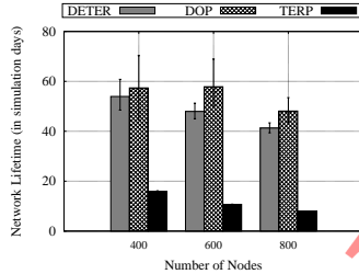
Fig. 11: Network lifetime
