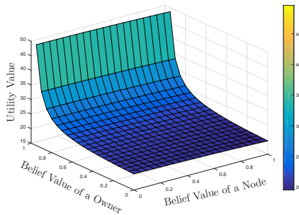
Fig. 4: Theoretical Analysis of Utility value
