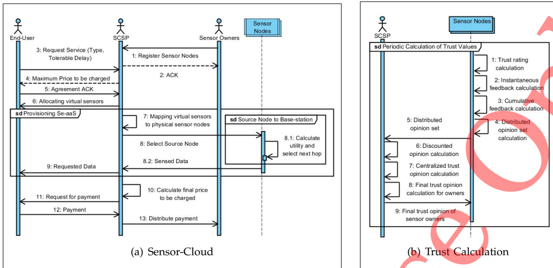
Fig. 3: Interaction Diagram of DETE
