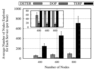
Fig. 7: Number of Nodes Explored
