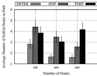
Fig. 13: Selfish Nodes in a Path
