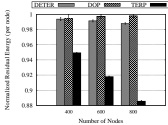
Fig. 10: Residual Energy of Nodes
