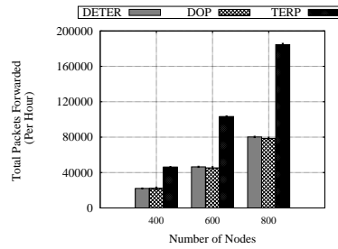
Fig. 8: Network Overhead
