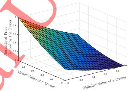
Fig. 5: Price with Varying Trust of Sensor-Owners
