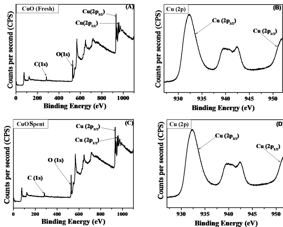
Figure 6. XPS spectra of (A) fresh CuO, (B) Cu present in CuO, (C) spent CuO, and (D) Cu present in spent CuO.
